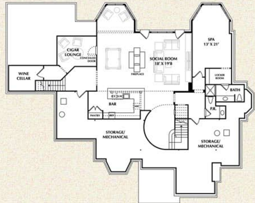
LOWER LEVEL PLAN
