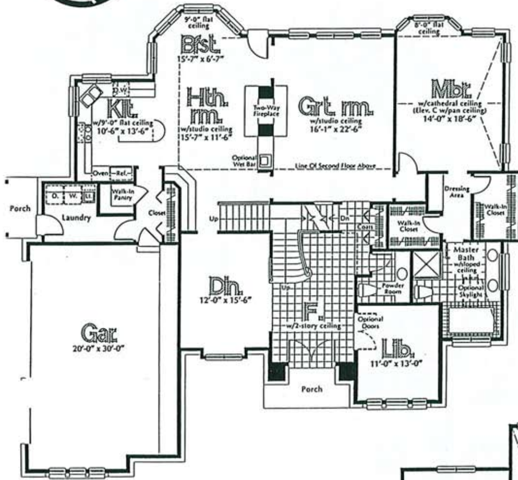
First Floor
