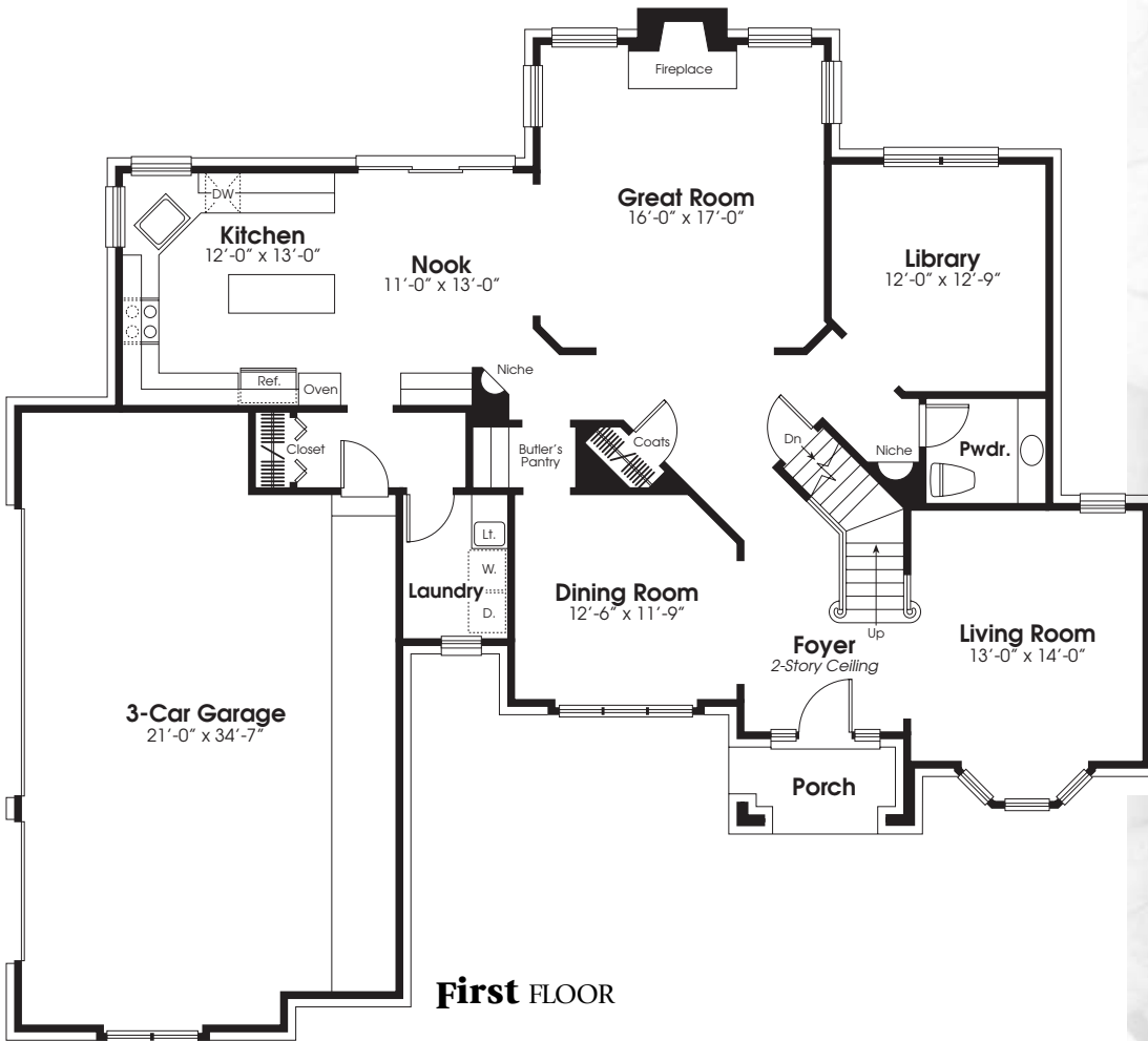
FLOOR PLAN DRAWN TO ELEVATION B
